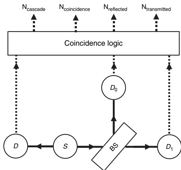
Fig. 1. Schematic diagram of the first experiment reported in the paper by Grangier et al. 4 demonstrating the indivisibility of the photon. S: Light source; BS: 50–50 beam splitter; D, D 0 , D 1 : Detectors; N_{\text{cascade}} : Number of excitations of the three-level cascade of the calcium atoms in the source S; N_{\text{coincidence}} : Number of times detector D 0 and D 1 fire within a time window relative to the excitation of the cascade; N_{\text{reflected}} : Number of photons reflected by the BS; N_{\text{transmitted}} : Number of photons transmitted by the BS. Solid lines: Flow of photons. Dashed lines: Flow of data.
