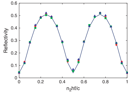
Fig. 11. EBCM simulation results (markers) for the reflectivity of a parallel plate ( n_1 = 1 , n_3 = 1.5 ) as a function of the optical thickness n_2hf/c for normal incidence of the incoming particles (see also Fig. 1.18 of Ref. [1]). The solid lines are the exact results of Maxwell's theory. 1 For the legend and simulation parameters, see Figure 10. For normal incidence, markers and solid lines for different polarizations coincide.
