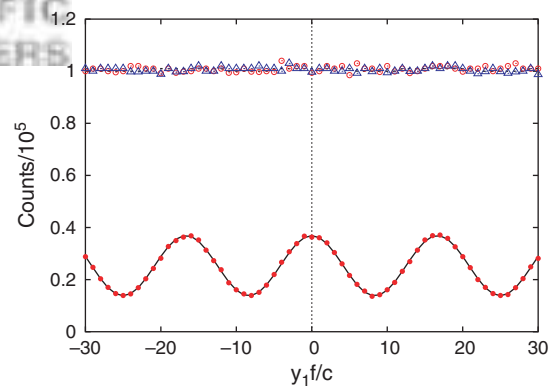
Fig. 26. Computer simulation data of the single-particle and two-particle counts for the HBT experiment depicted in Figure 25. Red open circles: EBCM results for the counts of detector D_0 . Blue open triangles: EBCM results for the counts of detector D_1 . Red closed circles: EBCM results for the coincidence counts. The dashed and solid lines are least-square fits of the predictions of wave theory to the EBCM data for the single detector and coincidence counts, respectively. Simulation parameters: N_{\text{tot}} = 2 \times 10^5 events per y_1/f/c -value, N_F = 40 , X = 100000c/f , d = 2000c/f , \gamma = \hat{\gamma} = 0.99 and N_p = 2 .
