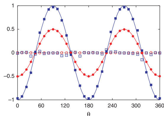
Fig. 23. Computer simulation data and quantum theoretical results for the single-particle and two-particle averages of the EPRB experiment depicted in Figure 22 as a function of \theta = \alpha_1 - \alpha_2 . The source emits particles with opposite polarization, uniformly distributed over the unit circle. Open circles and squares: Eq. (48) and (49), respectively; Closed squares: Eq. (50) Closed circles: Eq. (51) for W = T_{\text{EPRB}} , that is by ignoring the time-tag data; Blue solid line: \hat{E}_{12}(\alpha_1, \alpha_2) = -\cos 2\theta ; Red solid line: E = -2 \cos 2\theta . Simulation parameters: 3 \times 10^5 pairs, T_{\text{EPRB}} = 1000 , W = 1 , d = 4 , \gamma = \hat{\gamma} = 0.99 and N_p = 1 . Note that the total number of pairs emitted by the source is about the same as the number of photons per station detected in the experiment reported in Ref. [35] (experimental data set called longdist35).
