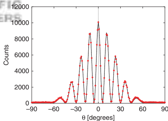
Fig. 13. Detector counts (circles) as a function of the angular detector position \theta as obtained from the EBCM simulation of the two-beam interference experiment depicted in Figure 12. The solid line is a least-square fit of the EBCM data to the prediction of wave theory, Eq. (36). The sources have a width a = c/f and are separated by a distance d = 5c/f and emit particles according to the current distribution Eq. (35). The source-detector distance X = 100c/f , see Figure 12. Simulation parameters: On average, each of the 181 detectors receives 10^4 messengers, \gamma = \hat{\gamma} = 0.99 and N_p = 500 .
