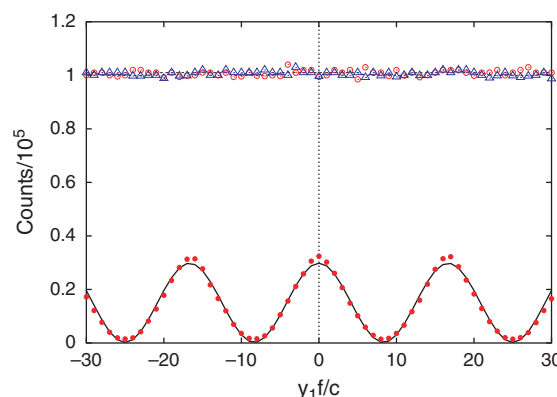
Fig. 27. Computer simulation data of the single-particle and two-particle counts for the HBT experiment depicted in Figure 25, generated by the same EBCM that produced the data of Figure 26 extended with the time-delay model Eq. (59). Red open circles: EBCM results for the counts of detector D_0 . Blue open triangles: EBCM results for the counts of detector D_1 . Red closed circles: EBCM results for the coincidence counts. The dashed and solid lines are least-square fits of the predictions of wave theory to the EBCM data for the single detector and coincidence counts, respectively. Simulation parameters: N_{\text{tot}} = 2 \times 10^5 events per y_1f/c -value, N_i = 40 , X = 100000c/f , d = 2000c/f , \gamma = \hat{\gamma} = 0.99 , N_p = 2 , W = 2/f , T_{\text{max}} = 2000/f and h = 8 .
