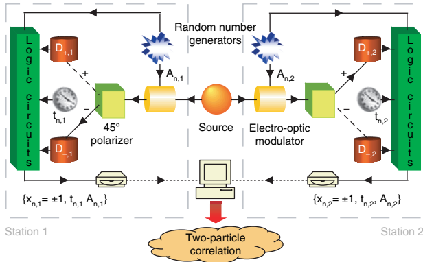
Fig. 22. Schematic diagram of an EPRB experiment with photons. 35
