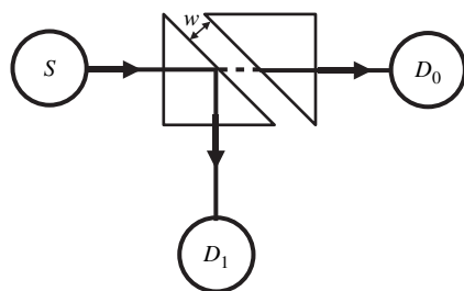
Fig. 20. Schematic diagram of the experimental setup for the photon tunneling experiment Ref. [30]. The hypotenuses of the identical prisms are separated from each other by a distance w .
