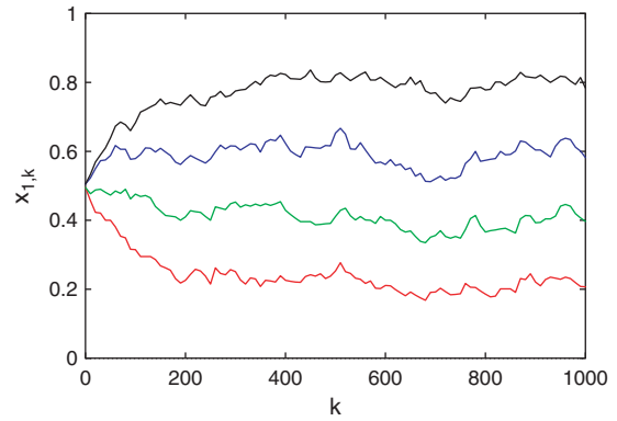
Fig. A.3. The first component x_{1,k} of the internal vector \mathbf{x}_k = (x_{1,k}, x_{2,k}) of a DLM that has two input ports to receive messages. A message arriving on input port 0(1) is represented by \mathbf{v}_k = (1, 0) ( \mathbf{v}_k = (0, 1) ). The probability that a message arrives on input port 0(1) is p_0 ( 1-p_0 ). Initially, the DLM is in the state \mathbf{x}_0 = (1/2, 1/2) and \gamma = 0.99 . Red line: p_0 = 0.2 ; Green line: p_0 = 0.4 ; Blue line: p_0 = 0.6 ; Black line: p_0 = 0.8 . This DLM estimates the frequency with which the messages arrive on input ports 0 and 1.
