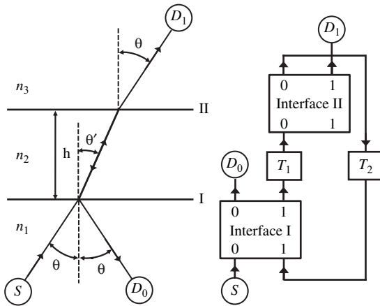
Fig. 9. Left: Diagram of the experiment to measure the reflection and refraction from a plane-parallel plate. In Maxwell's theory the source emits plane waves and the amount of energy in the reflected and transmitted light wave is recorded by detectors D_0 and D_1 , respectively. Right: In the EBCM, the source emits particles which are either reflected or transmitted by the interface I. In the latter case the particle travels to interface II where it is transmitted or reflected. In the latter case the particle travels back to interface I. The time-of-flights to travel from interface I to interface II and back again are T_1 and T_2 , respectively. The detectors D_0 and D_1 count the number of particles that are reflected or transmitted by the parallel plate, respectively.
