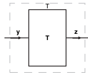
Fig. 14. Diagram of a processing unit that performs an event-based simulation of wave plates. Compared to the generic diagram Figure 4, the DLM stage and the output stage are missing. The solid lines represent the input and output ports of the device. The presence of a message is indicated by an arrow on the corresponding port line. The transformation matrices T for the HWP and QWP are given by Eqs. (41) and (42), respectively.
