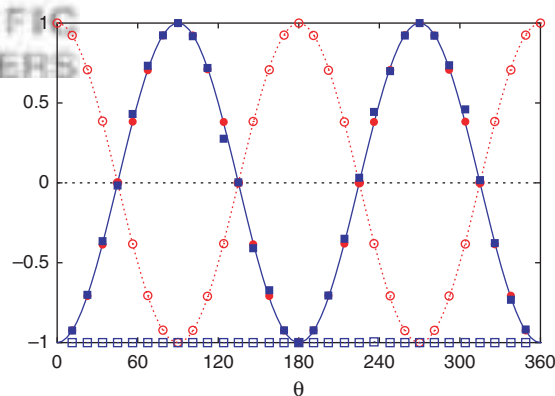
Fig. 24. Computer simulation data and quantum theoretical results for the single-particle and two-particle averages of the EPRB experiment depicted in Figure 22 as a function of \theta = \alpha_1 - \eta_1 with \alpha_2 = 0 . Same as in Figure 23 except that the source emits particles with P ( \eta_1 = 0 ) and S ( \eta_2 = \pi/2 ) polarization only. Open circles and squares: Eq. (48) and (49), respectively; Closed squares: Eq. (50); Closed circles: Eq. (51) for W = T_{\text{EPRB}} , that is by ignoring the time-tag data; Blue solid line: \hat{E}_{12}(\alpha_1, \alpha_2) = \cos 2(\alpha_1 - \eta_1) \cos 2(\alpha_2 - \eta_2) = -\cos 2\theta . Simulation parameters: Same as in Figure 23.
