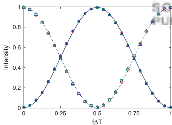
Fig. 15. EBCM simulation results for the number of particles registered by detectors D_0 (solid markers) and D_1 (open markers), divided by the total count of detected particles, as a function of the difference \Delta T = (T_0 - T_1(x)) between the time-of-flight in the lower and upper arm of the MZI, respectively. The solid and dashed lines are the exact results of Maxwell's theory for the normalized intensities at D_0 and D_1 , respectively. Simulation parameters: 10^4 events per pair of open or closed markers, \gamma = \hat{\gamma} = 0.99 . The markers for different polarizations (for the legend, see Fig. 10) coincide, in agreement with Maxwell's theory.
