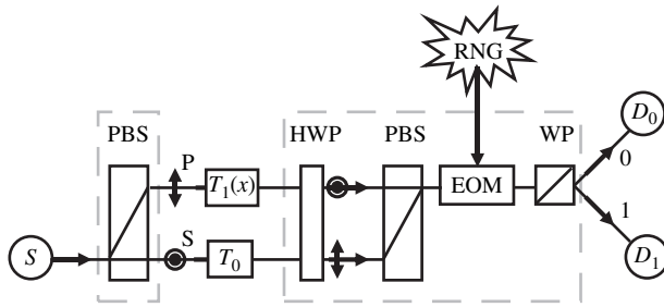
Fig. 16. Schematic diagram of the experimental setup for Wheeler's delayed-choice experiment with single photons. 28 PBS: Polarizing beam splitter; HWP: Half-wave plate; EOM: Electro-optic modulator; RNG: Random number generator; WP: Wollaston prism (=PBS); D_0 , D_1 : Detectors. The EBCM replaces the physical devices by the corresponding message-processing units.
