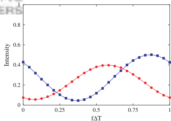
Fig. 19. The number of particles registered by detectors D 0 and D 1 divided by the total count of detected particles as a function of the time-of-flight difference \Delta T for \theta_0 = \pi/3 , \theta_1 = \pi/4 , and \theta_2 = \pi/8 , as obtained from the EBCM simulation of the quantum eraser experiment depicted in Figure 18. Circles: Intensity measured by D 0 ; Squares: Intensity measured by D 1 ; Solid red (blue) line: Intensity measured by D 0 ( D 1 ) as obtained from Maxwell's theory, see Eq. (44) (Eq. (45)). Simulation parameters: 10^4 events, \gamma = \hat{\gamma} = 0.99 and N_p = 1 .
