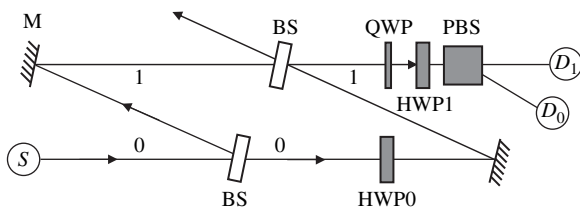
Fig. 18. Schematic diagram of the experimental setup for the quantum eraser experiment with photons studied in Ref. [29]. Moving the mirror labeled M changes the difference \Delta T between the time-of-flight in the lower and upper arm of the interferometer.
