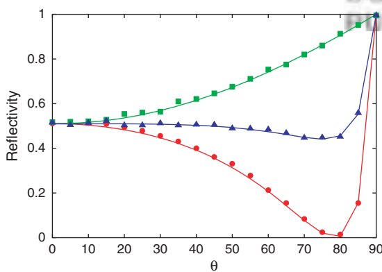
Fig. 10. EBCM simulation results (markers) for the reflectivity of a parallel plate ( n_1 = 1 , n_2 = 3 , h = c/4fn_2 , n_3 = 1.5 , corresponding to a quarter-wave plate) as a function of the angle of incidence of the incoming particles. The solid lines are the exact results of Maxwell's theory. 1 Green markers and lines: \xi = 0 (S-polarization); Blue markers and lines: \xi = \pi/4 (S+P polarization); Red markers and lines: \xi = \pi/2 (P-polarization). Simulation parameters: 10^4 events per marker, \gamma = \hat{\gamma} = 0.99 and N_p = 1 .
