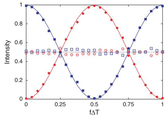
Fig. 17. EBCM simulation results (markers) for the Wheeler delayed-choice experiment depicted in Figure 16. The number of particles registered by detectors D_0 and D_1 divided by the total count of detected particles, as a function of the difference \Delta T = (T_0 - T_1(x)) between the time-of-flight in the lower and upper arm of the interferometer, respectively. Open circles: Intensity measured by D_0 for \theta_{\text{EOM}} = 0 ( r_n = 0 ); Open squares: Intensity measured by D_1 for \theta_{\text{EOM}} = 0 ; Closed circles: Intensity measured by D_0 for \theta_{\text{EOM}} = \pi/4 ( r_n = 1 ); Closed squares: Intensity measured by D_1 for \theta_{\text{EOM}} = \pi/4 ; Dashed line: Intensities measured by D_0 and D_1 as obtained from Maxwell's theory for \theta_{\text{EOM}} = 0 ; Solid red (blue) line: Intensity measured by D_0 ( D_1 ) as obtained from Maxwell's theory for \theta_{\text{EOM}} = \pi/4 . Simulation parameters: 2600 emitted events per pair of open/closed markers, \gamma = \hat{\gamma} = 0.99 and N_p = 1 . The actual counts (= 1300 \times intensities) are in good quantitative agreement with the experimental results reported in Ref. [28].
