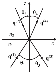
Fig. 3. Refraction and reflection at a boundary between two dielectric materials with indices of refraction n_1 and n_2 . The vectors \mathbf{q}^{(1)} , \mathbf{q}^{(2)} , \mathbf{q}^{(3)} , and \mathbf{q}^{(4)} lie in the x - z plane.
