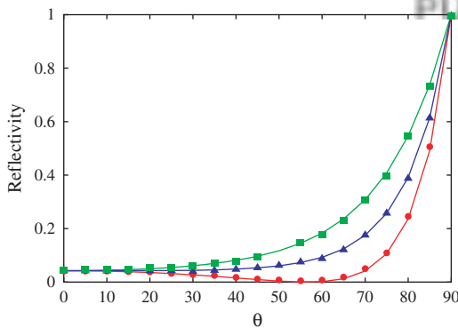
Fig. 7. EBCM simulation results (markers) for the reflectivity of an interface between vacuum ( n_1 = 1 ) and glass ( n_2 = 1.52 ) as a function of the angle of incidence of the incoming particles (see also Fig. 1.12 of Ref. [1]). The solid lines are the exact results of Maxwell's theory. 1 Green markers and lines: \xi = 0 (S-polarization); Blue markers and lines: \xi = \pi/4 (S+P polarization); Red markers and lines: \xi = \pi/2 (P-polarization). Simulation parameters: 10^4 events per marker, \gamma = \hat{\gamma} = 0.99 and N_p = 1 .
