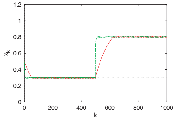
Fig. A.1. The internal state of the DLM as a function of the number of input events k . Red line: DLM defined by the update rule Eq. (A.2). Green line: DLM defined by the update rule Eqs. (A.3) and (A.4).
