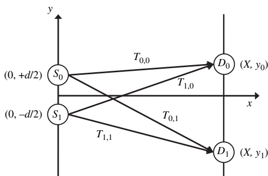
Fig. 25. Schematic diagram of a HBT experiment. Single photons emitted from point sources S_0 and S_1 are registered by two detectors D_0 and D_1 . The time-of-flight for each of the four possible paths from source S_m to detector D_n is denoted by T_{m,n} where m, n = 0, 1 .
