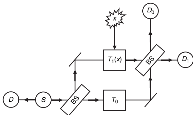
Fig. 2. Schematic diagram of the second experiment reported in the paper by Grangier et al. 4 demonstrating that photons build up an interference pattern one by one. S: Light source; BS: 50–50 beam splitter; T_0 : Fixed time-of-flight; T_1(x) : Variable time-of-flight controlled by the external variable x ; D, D 0 , D 1 : Detectors. For clarity, the coincidence logic (see Fig. 1) has been omitted.
