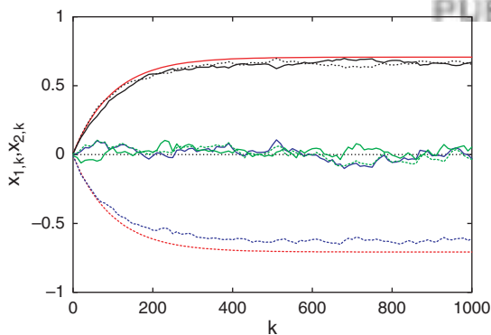
Fig. A.2. The two components of the internal vector \mathbf{x}_k = (x_{1,k}, x_{2,k}) as a function of the number of received events k for four different input messages \mathbf{e}_k = (1, -1)/\sqrt{2} (red lines) with statistical average (1, -1)/\sqrt{2} , \mathbf{e}_k = (r_k^{1/2}, (1-r_k)^{1/2}) (black lines) with statistical average (2/3, 2/3) , \mathbf{e}_k = (\cos \pi r_k, -\sin \pi r_k) (blue lines) with statistical average (0, 2/3) , and \mathbf{e}_k = (\cos 2\pi r_k, \sin 2\pi r_k) (green lines) with statistical average (0, 0) , 0 \leq r_k < 1 being uniform pseudo-random numbers. Solid lines: x_{1,k} ; Dashed lines: x_{2,k} . In all cases \mathbf{x}_0 = (0, 0) and \gamma = 0.99 .
